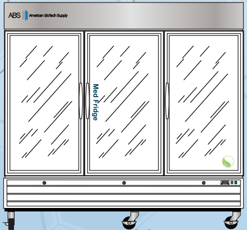
PH-ABT-HC-S72G Pharmacy Refrigerator Upright Glass Door Standard 72 CF
